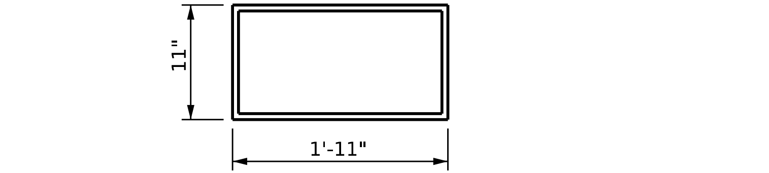
E5 ( _REQ'D ) PLAN VIEW OF ELASTOMERIC BEARING
