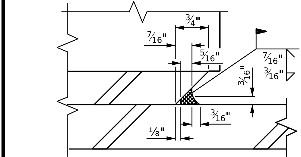
DETAIL "A"
