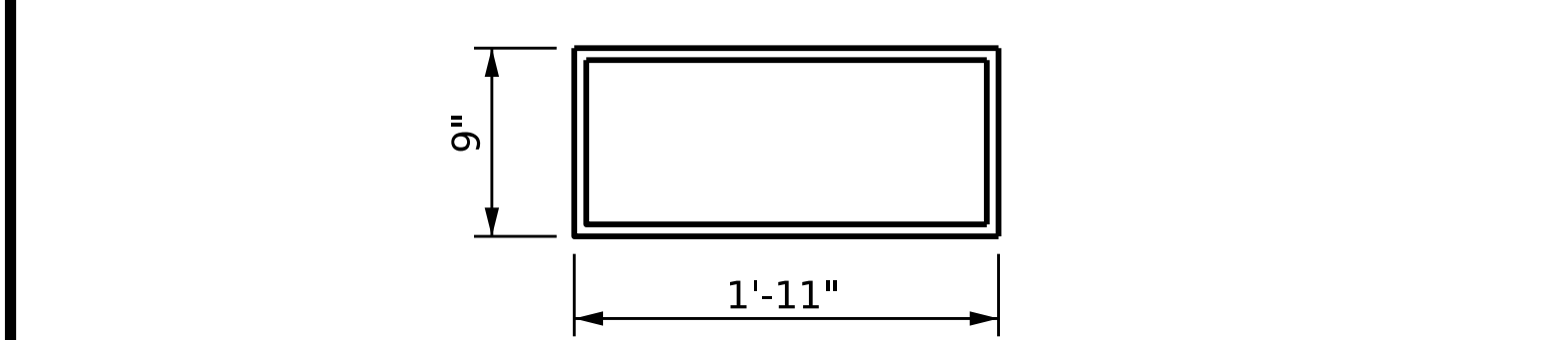
E4 ( _REQ'D ) PLAN VIEW OF ELASTOMERIC BEARING
